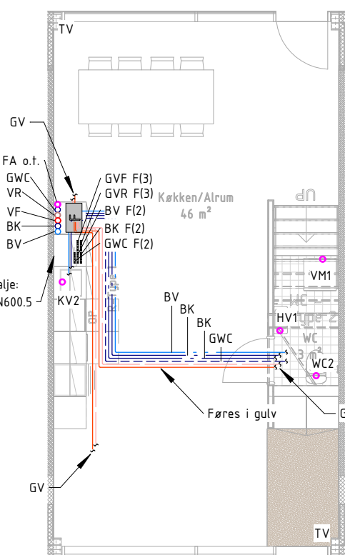
VVS ETAGE 00 Type R-3-C
